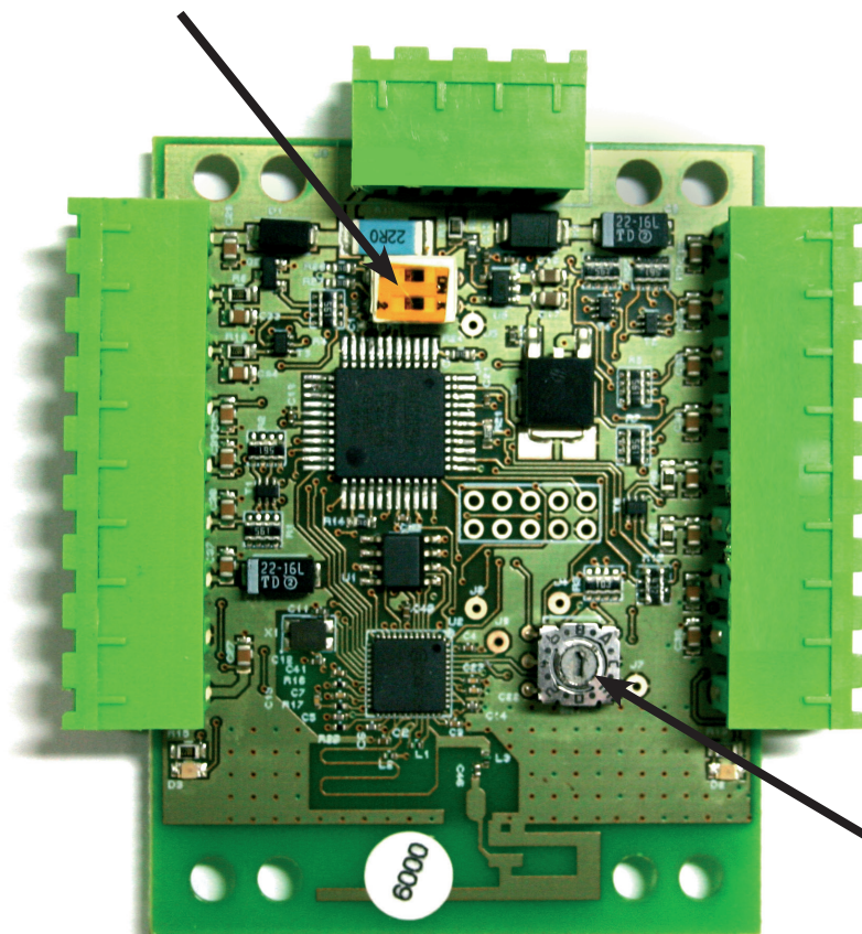
Interface PCB
