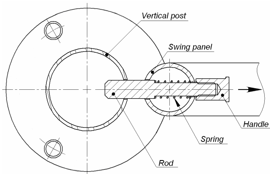
Fig. 15 Installation of the stopper unit rod
