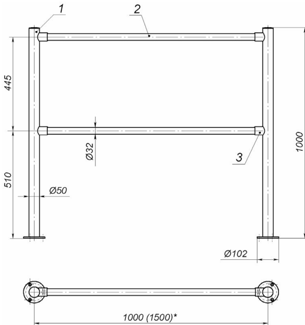
Fig. 2 Stationary railing section without filler panel: 1 – vertical post; 2 – rail; 3 – coupling fitting
