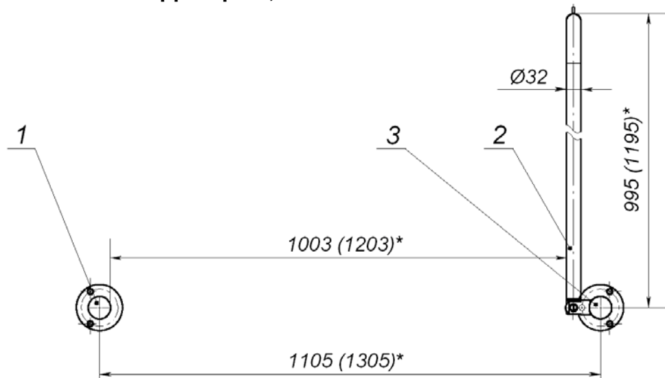
Fig. 5 Rotary railing section with mechanical BD in the open state: 1 – vertical post; 2 – swing panel; 3 – support post
