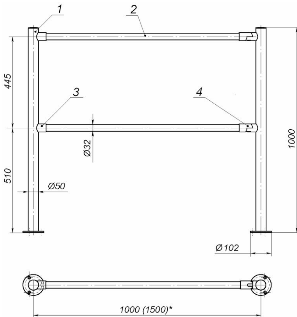
Fig. 3 Stationary railing section without filler panel and with adjustable coupling fittings: 1 – vertical post; 2 – rail; 3 – coupling fitting; 4 – adjustable coupling fitting
