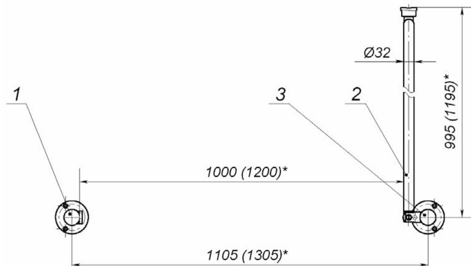
Fig. 7 Automatic rotary railing section with electromagnetic BD in the open state: 1 – post with electromagnetic BD; 2 – swing panel; 3 – support post (* – see Table 4 for variants)
