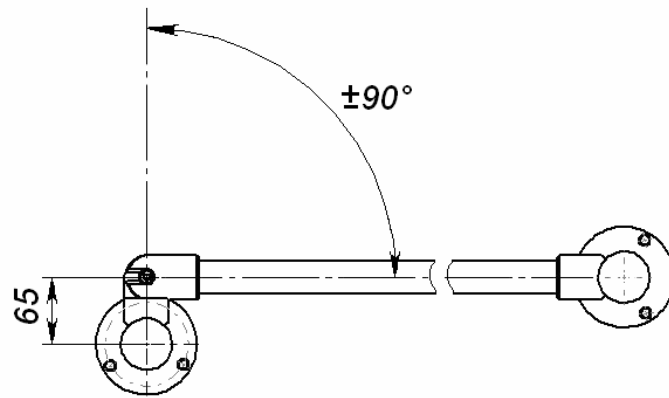
Fig. 12 Available turning angles for BH-01 0-01 adjustable coupling fitting
