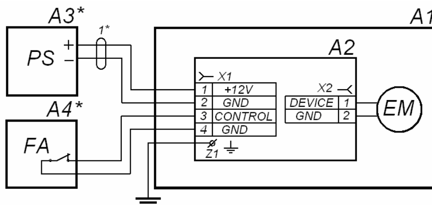
Fig. 16 Electric circuit scheme of the post with electromagnetic BD (see Table 5 for the list of elements)
